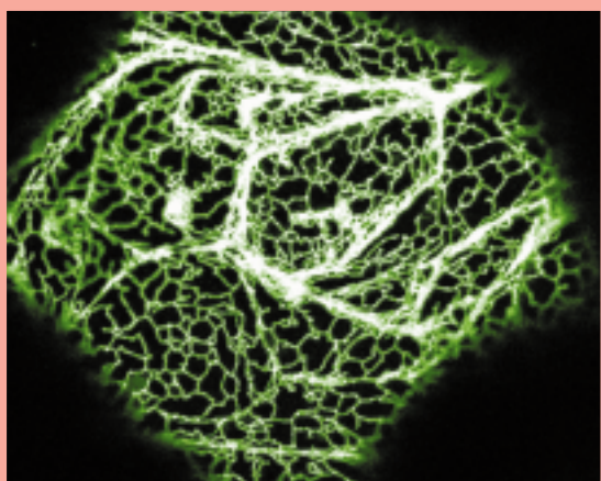
Figure 2 Fluorescent cortical ER in a PVX.sp-GFP-K infected Nicotiana clelandii epidermal cell.
