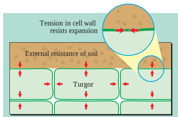
Figure 1 Schematic diagram showing pressures acting in the epidermis of a root growing in soil.
