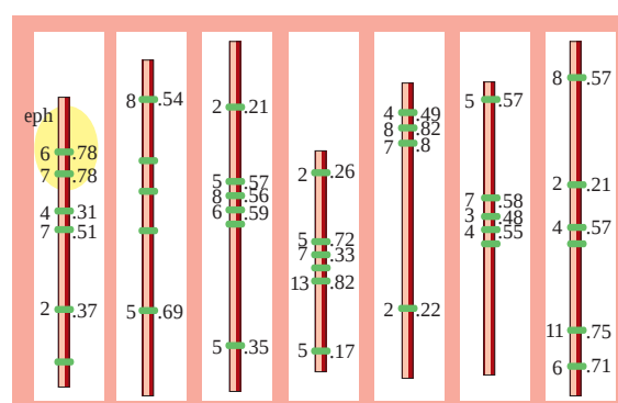
Figure 1 Allele numbers and diversity indices at chosen SSRs - 67 genotypes.
