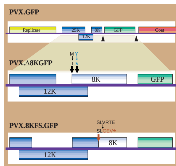
Figure 1 Viral genomes of 'wild-type' and mutant forms of PVX.GFP.
