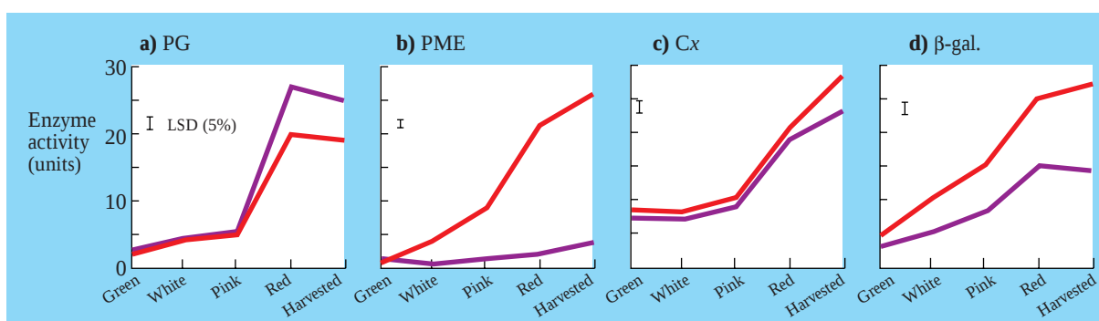
Figure 2 Activities of PG (a), PME (b), Cx(c) and β-gal (d) in ripening drupelets of Glen Prosen (red) and Glen Clova (purple).
